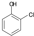
2-Chloro-phenol
