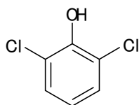
2,6-Dichloro-phenol
